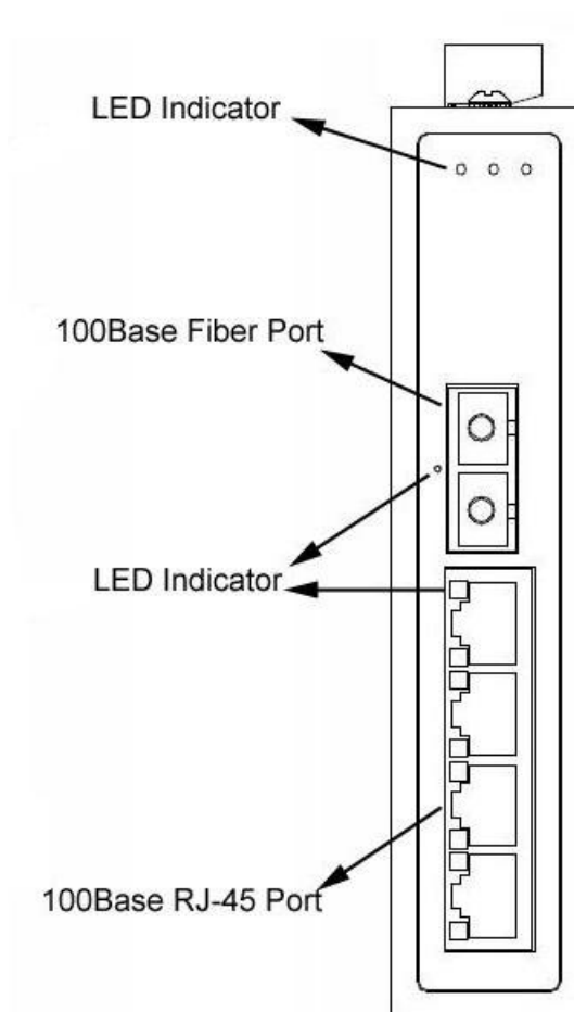
Front Panel of the 4-port 10/100TX + 1 100FX Industrial Switch
