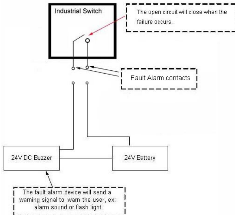
Wiring the Fault Alarm contacts to an external warning device
